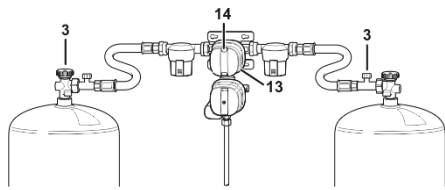
Fig. 115: Gas pressure regulator set
