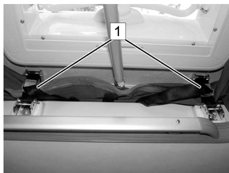
Fig. 155: Roof locking mechanisms
