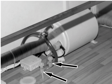
Fig. 139: Drain valves
