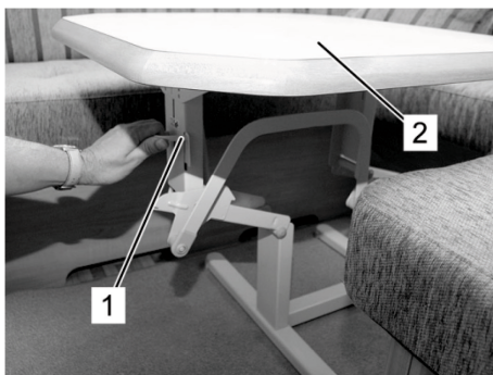
Fig. 141: Table with table lift frame
